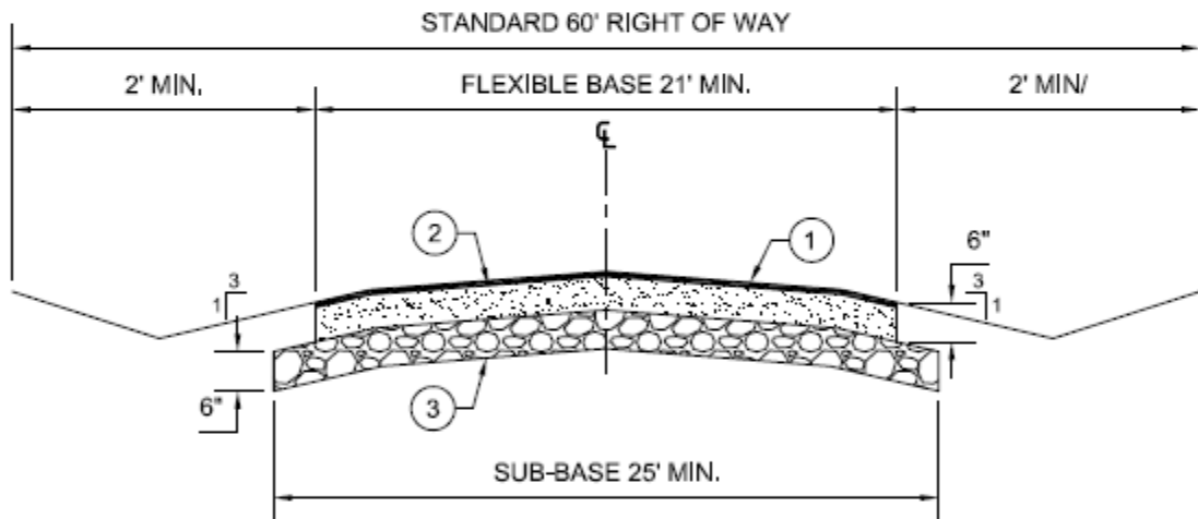
ONE TRAVEL LANE & TWO PARKING LANES N.T.S.
